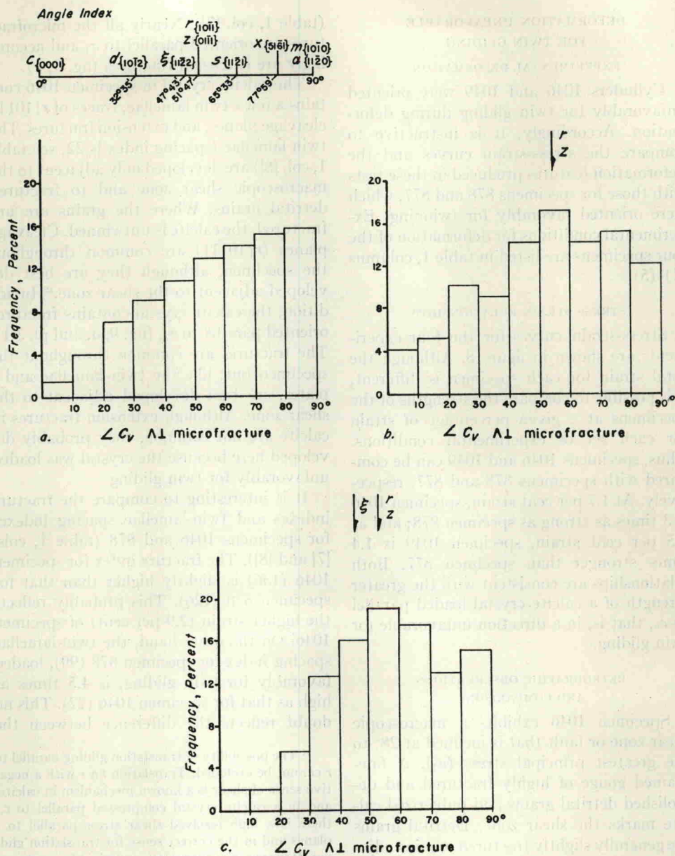
FIG. 6.—Histograms of distribution of angles between normal to microfractures and c_v in host quartz grains. a, random distribution (Bloss, 1957):
